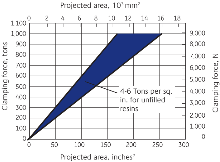
Figure 6-4 Clamping force for Ultem resins.
